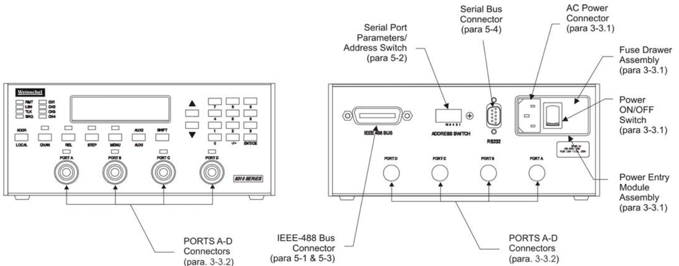
Figure 1. Front & Rear Panel Connectors
