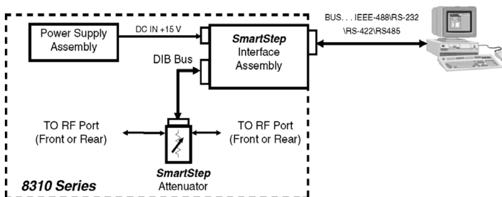
Figure 5. 8310 Series Simplified Block Diagram
