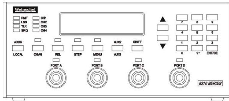
Figure 2. 8310 Series Front Panel
